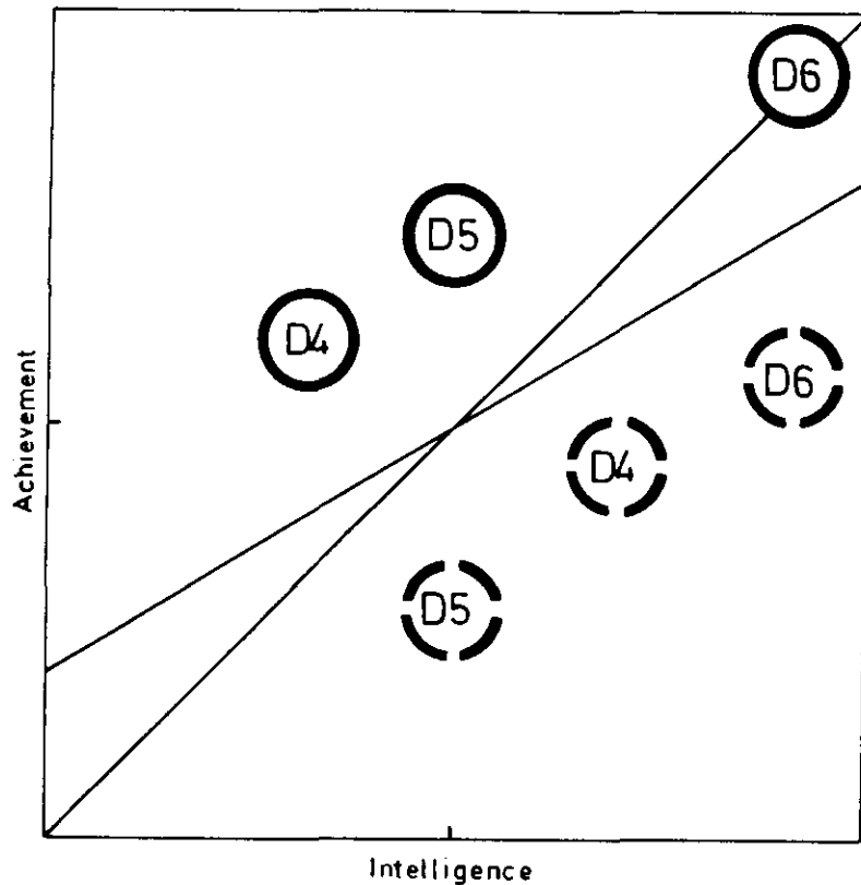
Fig. 1:3. A comparison between the method of difference and the method of regression. The unbroken circles indicate groups of achievers or overachievers, and the broken circles underachievers. The legends indicate the variant of the method of difference to which reference is made.
