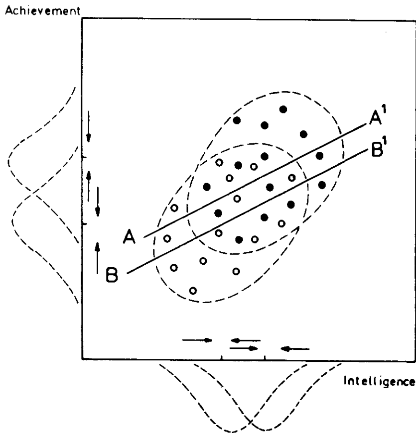
Fig. 1:5. Illustration of variant R3. The individuals are divided according to a certain background variable into groups A and B. The regression lines of these groups and marked A - A 1 and B - B 1 respectively. ● = the positions of the individuals in group A, ○ = the positions of the individuals in group B.
