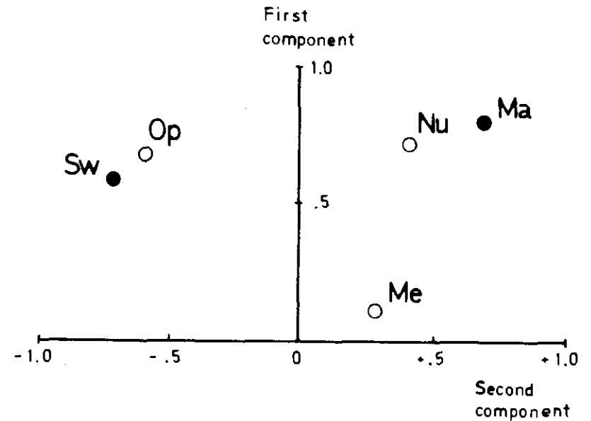
Fig. 4:2. Canonical weights. Intelligence tests and school marks.
